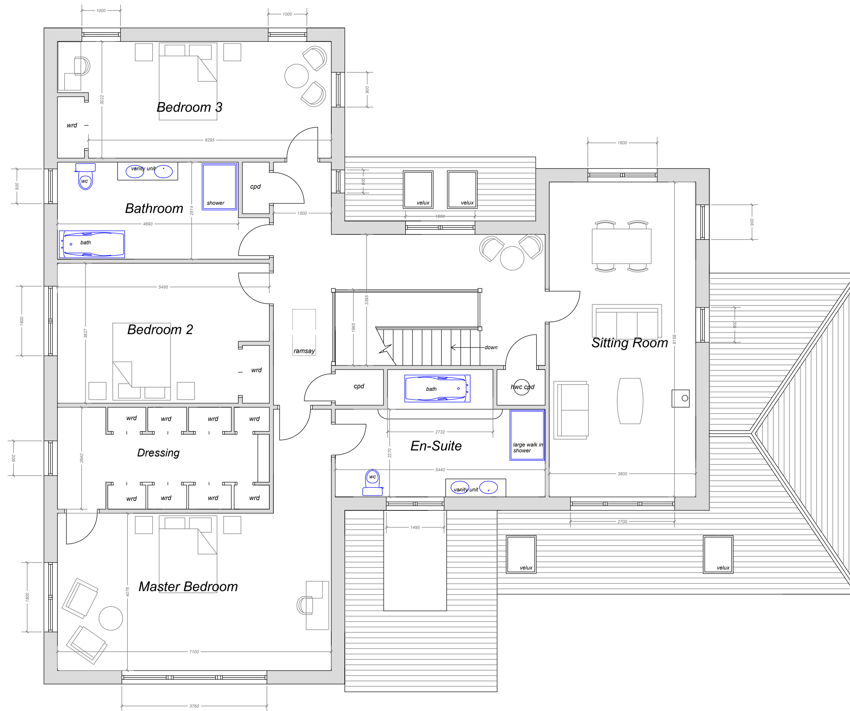
FIRST FLOOR PLAN (139m2)
